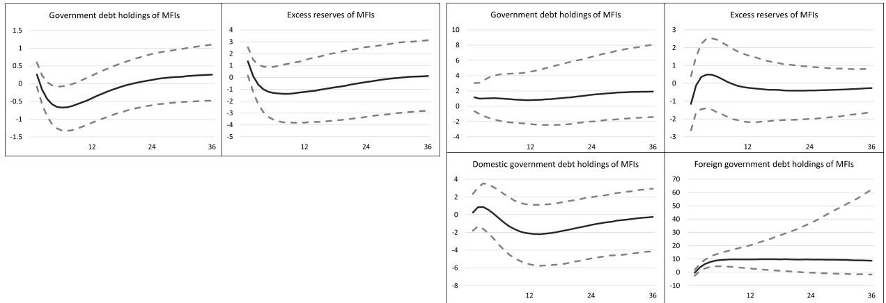
Figure 4: Transmission via banking sector (I) (a) Euro area (b) Latvia
