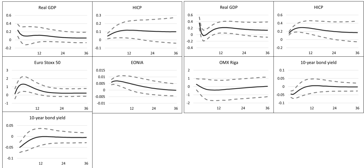
Figure A6: Robustness check - using QE factor of Altavilla et al. (2019) (a) Euro area (b) Latvia
