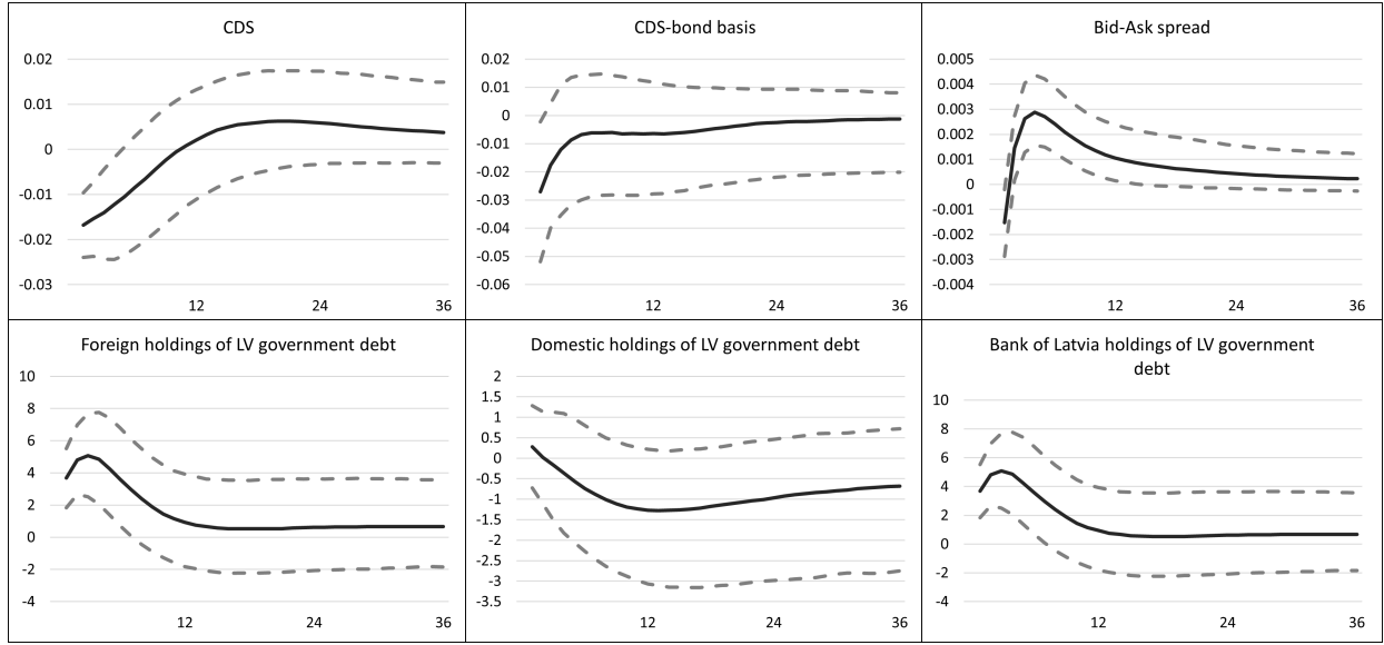
Figure 3: Transmission to sovereign yields Latvia
