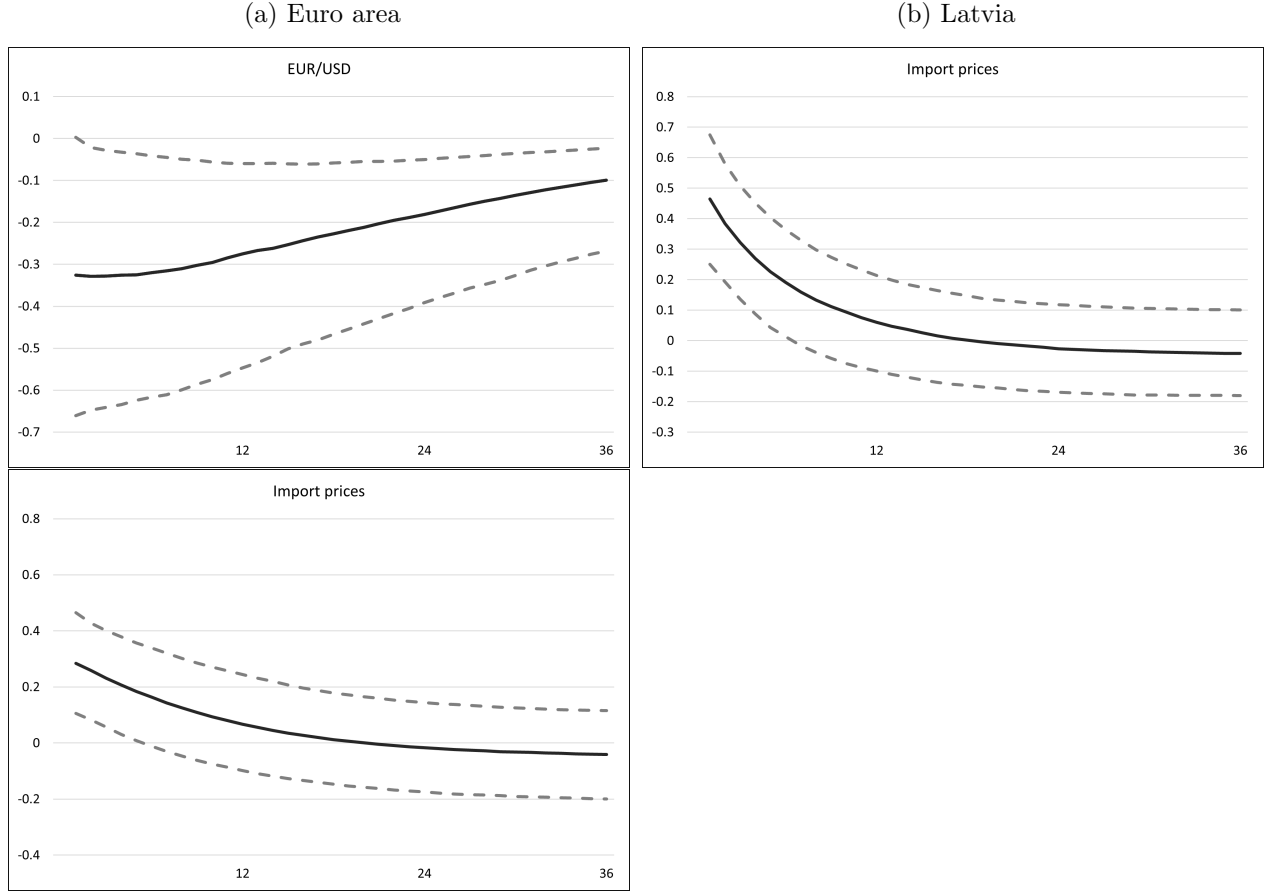
Figure 2: Exchange rate channel
