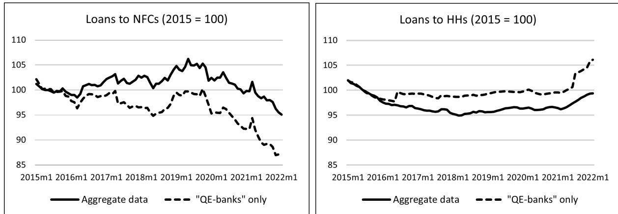
Figure 6: Lending dynamics: "QE-banks" vs. aggregate data Latvia
